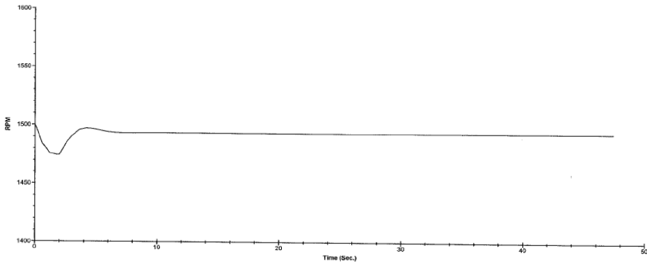
Fig. 12. Speed response after load shedding
