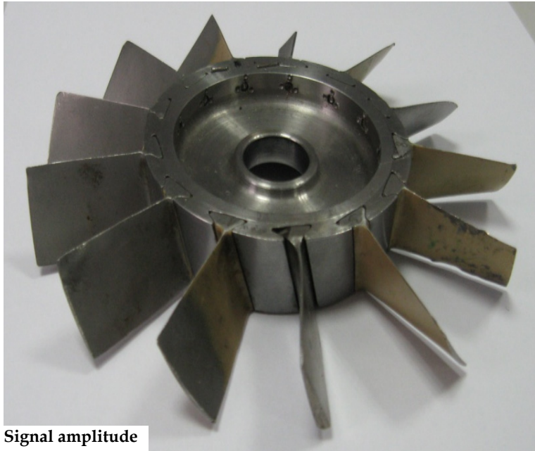
Fig. 8. View of the turbine disc with blades
